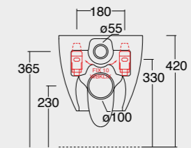
Cod. 45000101 Vaso sospeso Wunder Wunder WC wall hung
